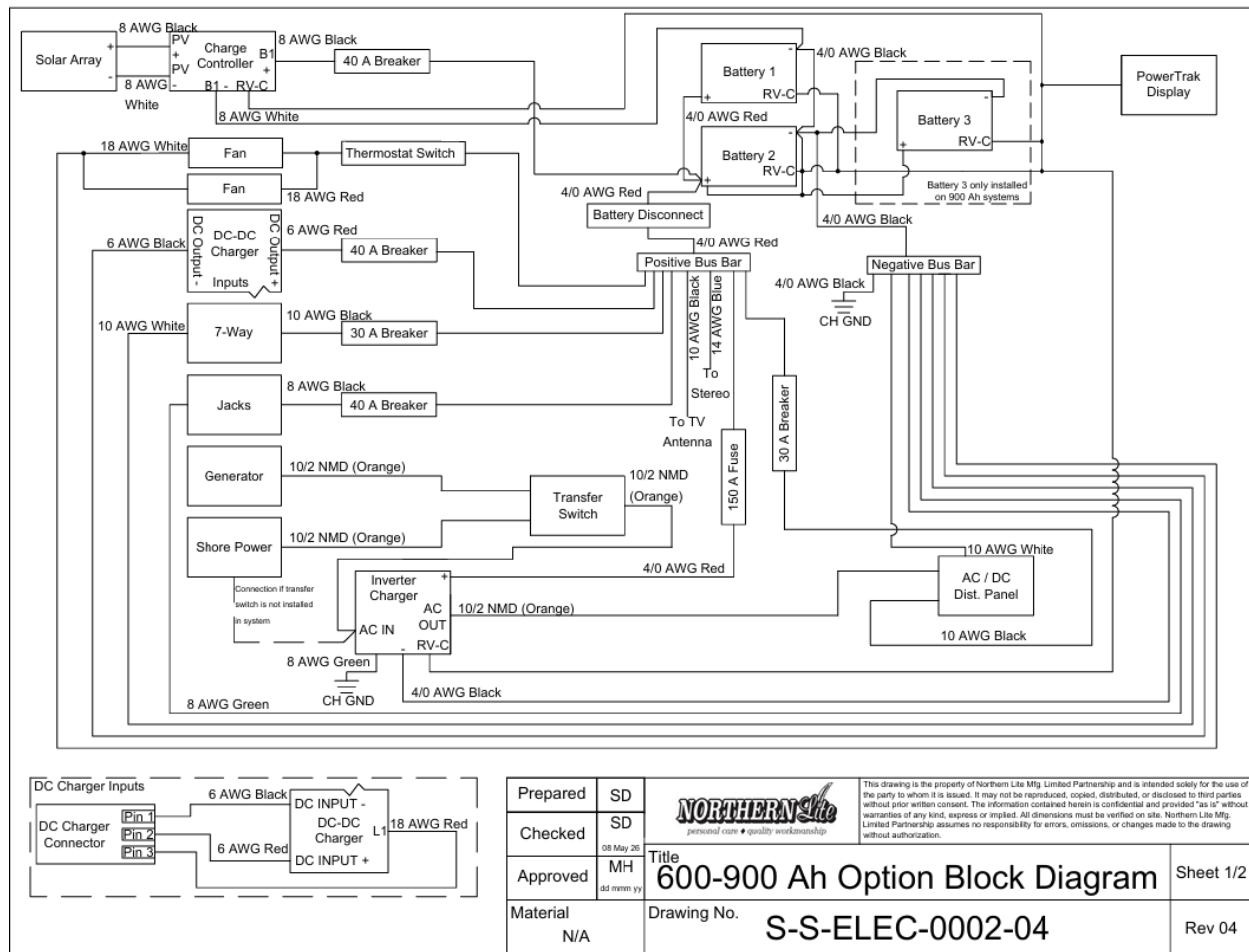
Figure 1 - Electrical Schematic
