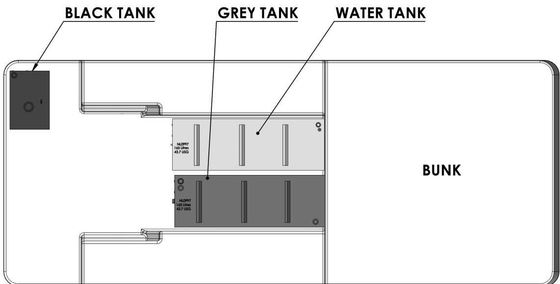
TOP VIEW OF CAMER BASEMENT SHOWING TANK LAYOUT
